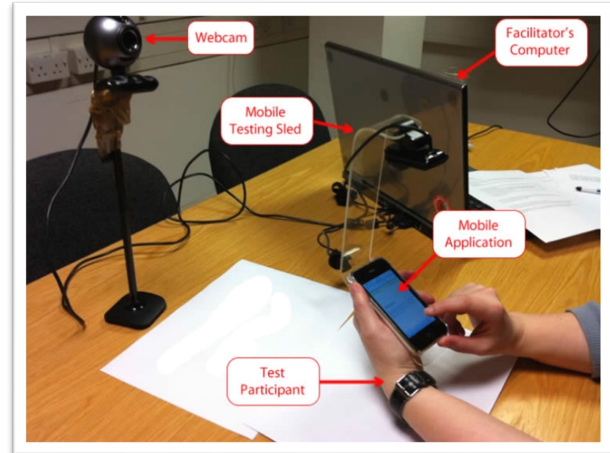
User test: walk-through
